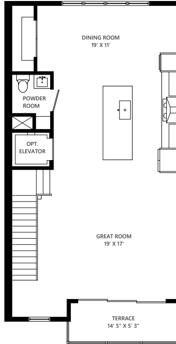
2nd Floor
