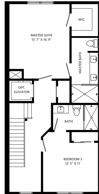
3rd Floor
