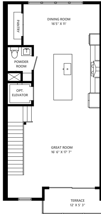
2nd Floor
