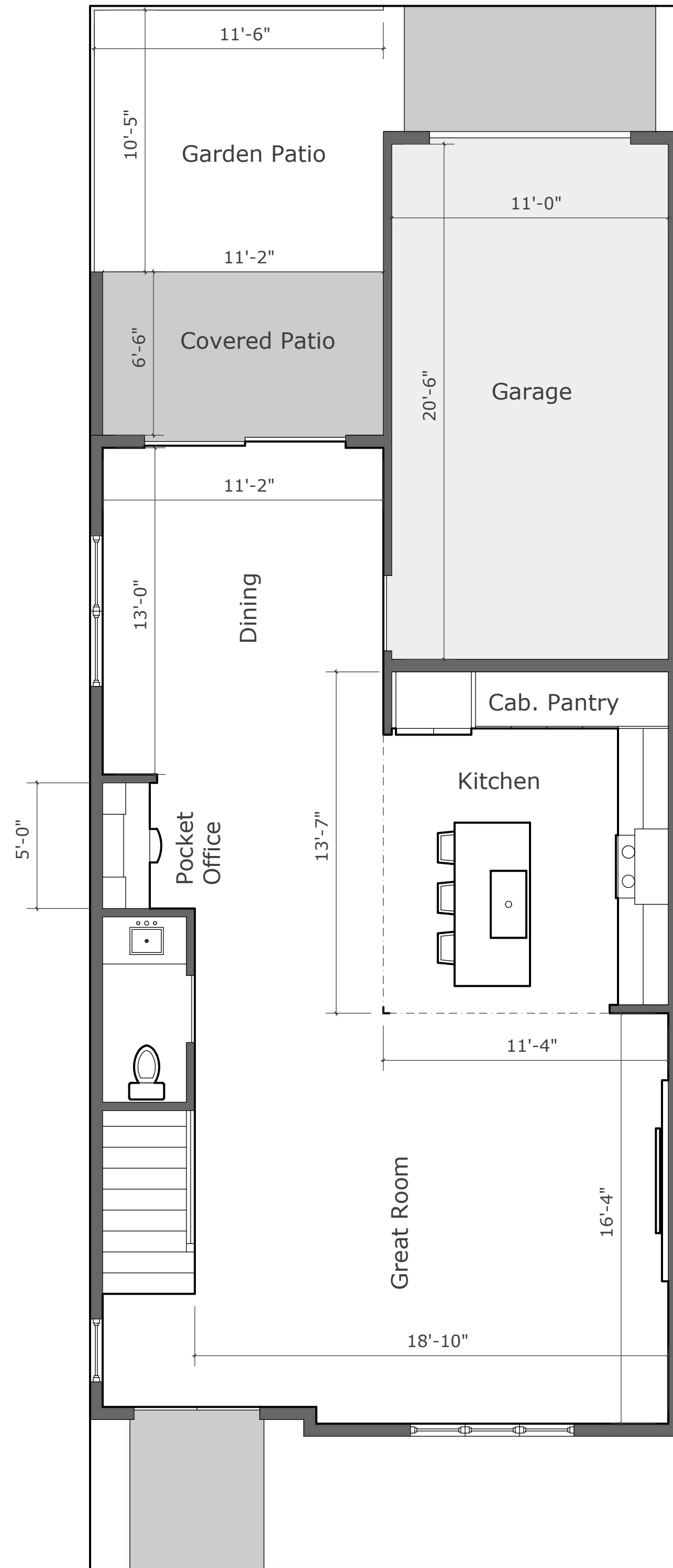
1st Floor
