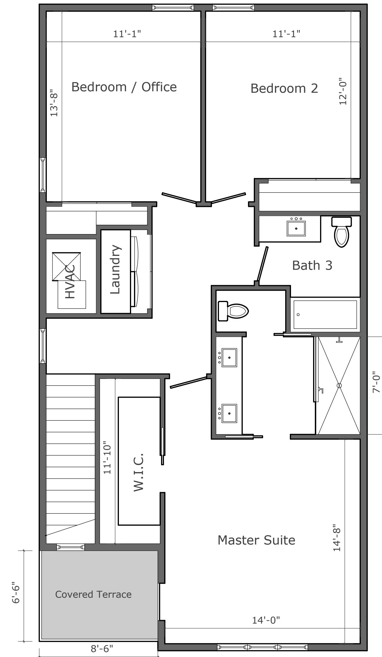
2nd Floor
