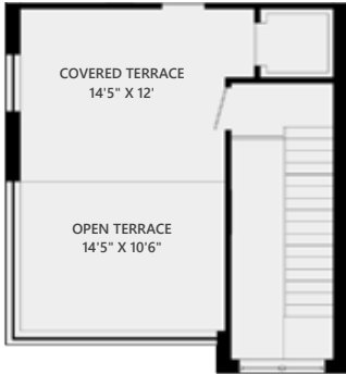
Optional 4th Floor with Rooftop Terrace
